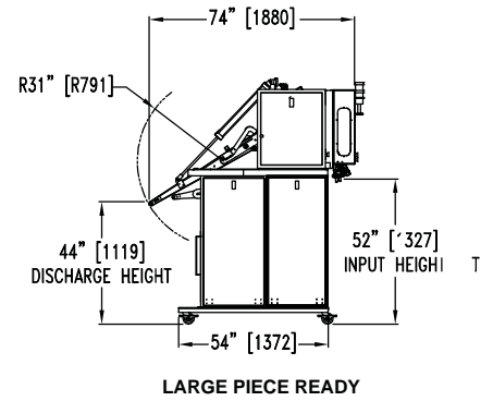
Left View
